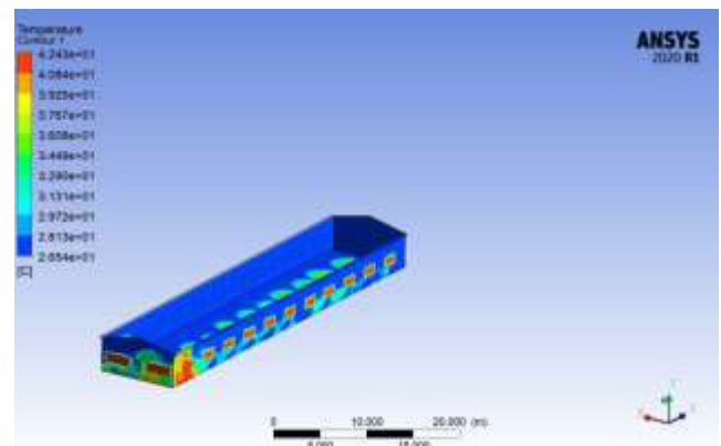
Figure 14. Temperature for poultry house with evaporator and exhaust fan
